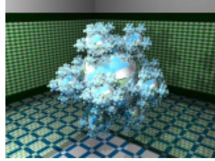
Figure 10: Sphere-Flake.
