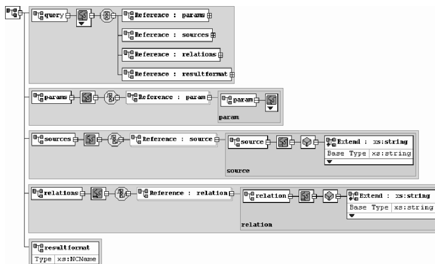
Fig. 1. The schema for general VQL queries
