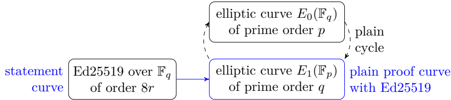
Figure 4: Plain cycle with Ed25519 as the statement curve.
