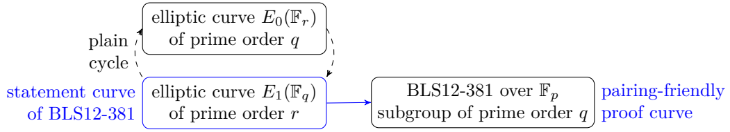
Figure 3: Plain cycle, one curve is a statement curve with the proof curve BLS12-381.
