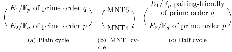
Figure 2: The three known types of cycles of curves.
