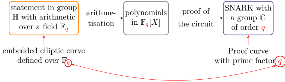
Figure 1: Relation between base field of the embedded curve and scalar field of the proof curve (adapted from [AEG23, Figure 3]).
