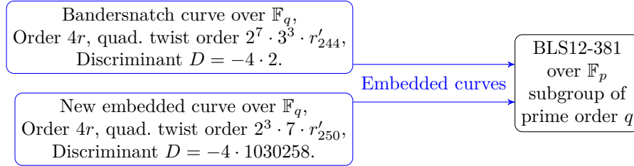
Figure 5: Two secure embedded curves for BLS12-381.
