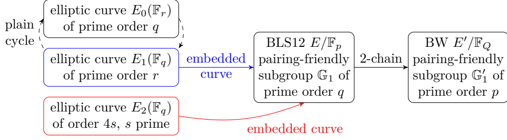
Figure 6: Plain embedded cycle and embedded curve associated to an inner BLS12 curve, and an outer curve forming a 2-chain.
