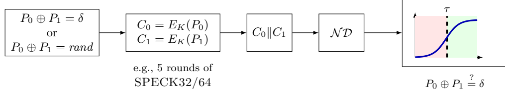
Figure 1: Neural Differential Distinguisher: Basic Training Pipeline. Given plaintexts P_0, P_1 with P_0 \oplus P_1 \in \{\delta, \text{rand}\} , encrypt under key K to obtain C_i = E_K(P_i) . The concatenation C_0 || C_1 is fed to \mathcal{ND} , which outputs a sigmoid score \hat{Y} \in [0, 1] ; thresholding at \tau yields a binary decision for P_0 \oplus P_1 = \delta (yes if \hat{Y} \geq \tau ). In the plot, the constant baseline for the negative class is shown in red and the sigmoid for the positive class in green ; the background halves visualize the threshold.
