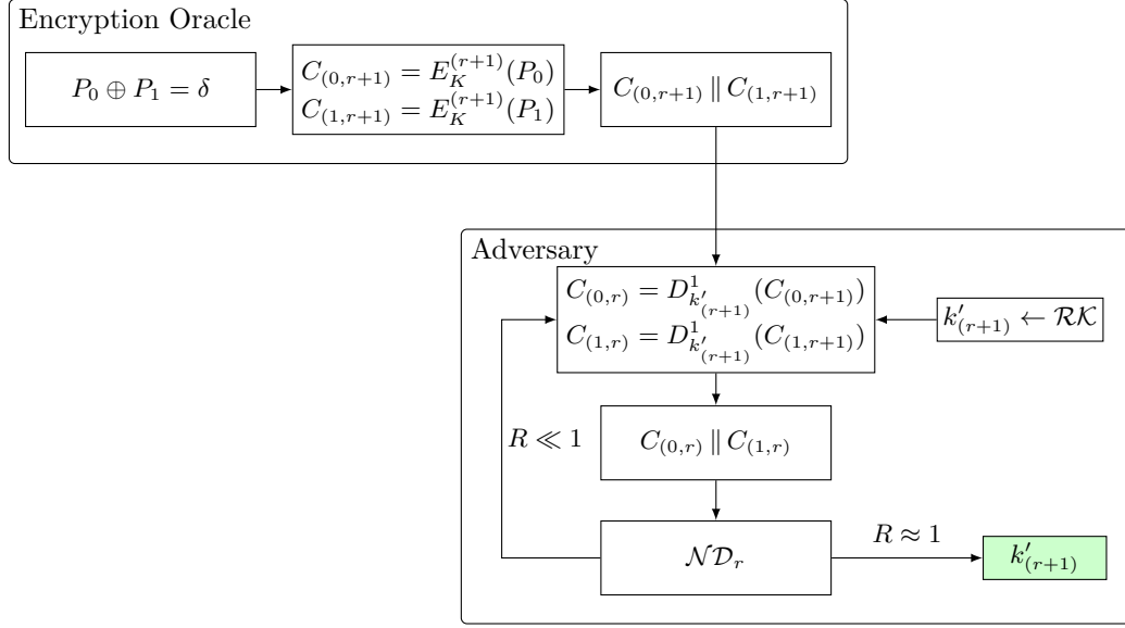
Figure 2: Neural Differential Distinguisher: Basic Key Recovery Pipeline. Let \mathcal{RK} denote the round-key space of the block cipher under scrutiny. An encryption oracle (with a secret master key K ) generates an (r+1) -round ciphertext pair with input difference \delta . The adversary decrypts round (r+1) using a key guess k'_{(r+1)} and feeds the result to a neural distinguisher \mathcal{ND}_r , which has been trained on the r -round ciphertext pair distribution. Key guesses k'_{(r+1)} producing distinguisher scores near 1 are output as candidates, following the wrong-key randomization hypothesis [Goh19].
