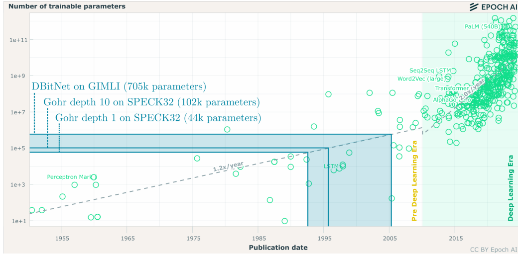
Figure 4: Adapted from [Epo23] with added data for Gohr’s \mathcal{ND}_{\text{Gohr}} on Table 6, and DBitNet on Table 14 from [BGHR23, Table 5].
