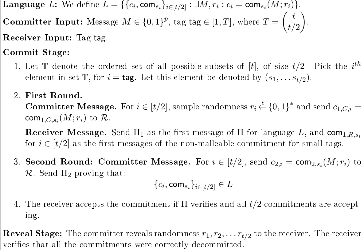
Figure 9: Round-Preserving Tag Amplification
