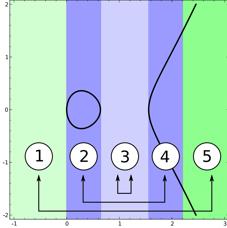
Figure 1: Wallpapering a real Montgomery curve
