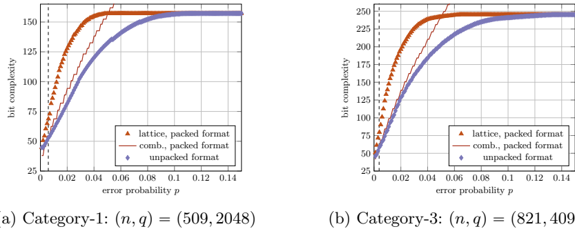
Fig. 6: Bit complexity of key recovery on NTRU in the symmetric error model.
