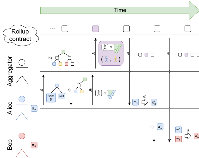
Fig. 1. The transfer protocol. In this example, Alice wants to send 5 coins to Bob. a) Alice starts by sending the hash of the the transaction batch, consisting of a single transaction of 5 coins to Bob, and a random salt to an aggregator. b) The aggregator then constructs a merkle tree consisting of Alice’s transaction batch hash and the transaction batch hashes of other senders. c) The aggregator sends the merkle proof of Alice’s transaction batch to Alice. d) Alice verifies the merkle proof and signs the merkle root together with the pre-determined extradata e . This signature is sent back to the aggregator. e) The aggregator collects the signatures from all senders, constructs the transfer block, and sends it to the rollup contract. f) Alice watches the blocks that are added to the rollup contract until the block containing her transaction is published. g) Alice updates her balance proof by adding her transaction batch, the salt and the merkle proof. h) Alice sends to Bob her updated balance proof. h) Bob updates his view of the rollup blocks. i) Bob updates his balance proof by merging it with the balance proof he received from Alice.
