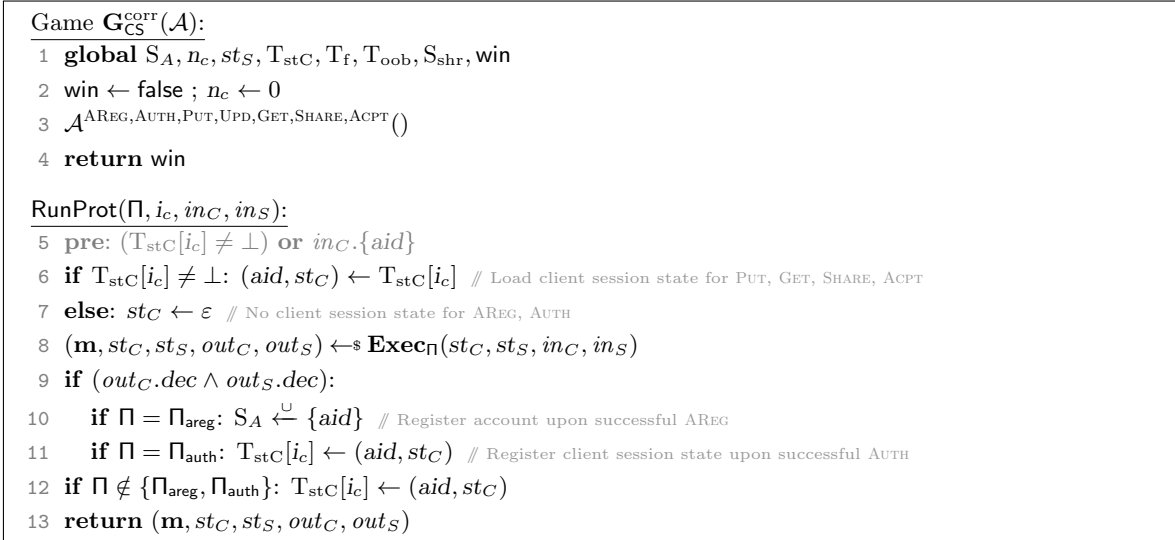
Figure 2: Correctness game \mathbf{G}_{\text{CS}}^{\text{corr}} for cloud storage scheme CS, with oracles given in Figure 3, and helper function RunProt used by oracles.
