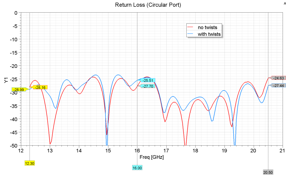
Figure 28. Simulated Return Loss S(1:1,1:1) , Final OMT
